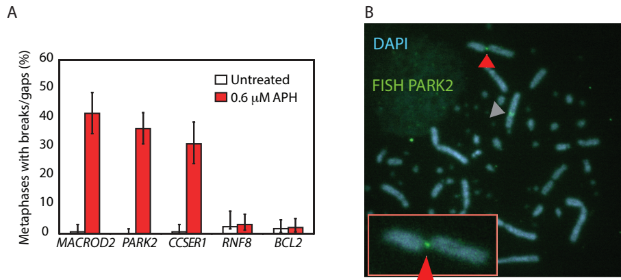
Figure 2. Peak regions from FANCD2 ChIP-seq form breaks on metaphase chromosomes after APH treatment. (A) Quantification of breaks or gaps at the indicated loci with or without 0.6 \mu M APH treatment for 16 h. BCL2 and RNF8 are control loci, which were not bound by FANCD2 in the ChIP-seq experiment. At least 170 metaphases were counted for each locus. (B) Representative image of metaphase spread from DT40 cells treated with 0.6 \mu M APH for 16 h. The FISH probe hybridizes to PARK2 , which is broken (close up image and red arrowhead). One allele of PARK2 is not broken (grey arrowhead).
